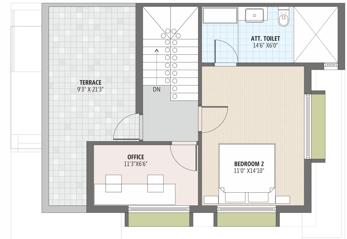
SECOND FLOOR
