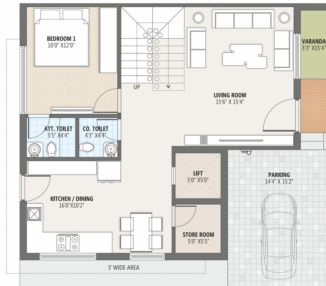
GROUND FLOOR
