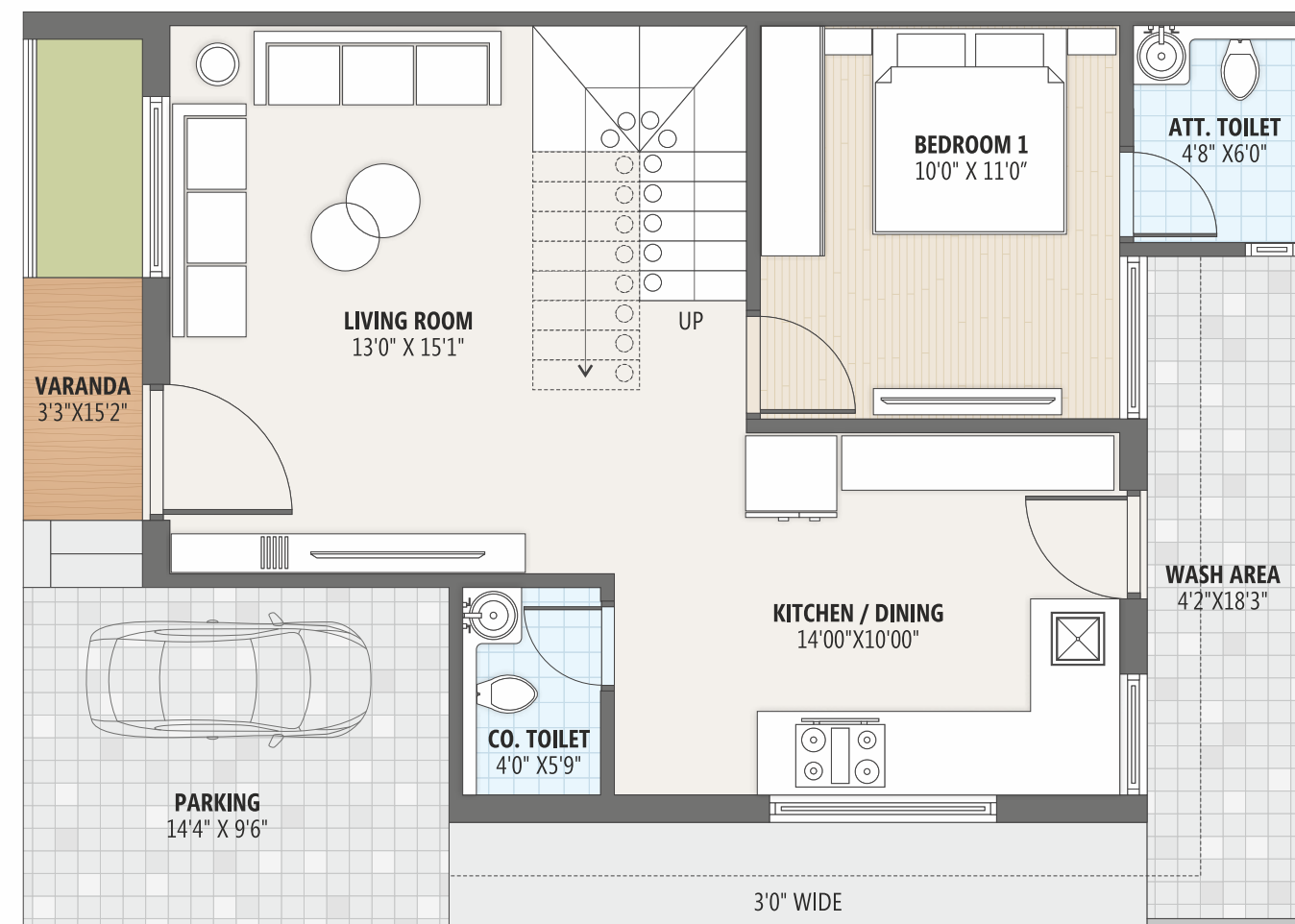
GROUND FLOOR
